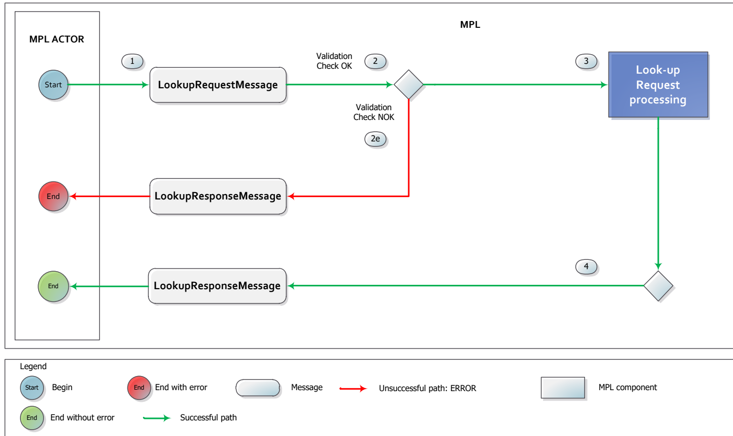
Figure 5 – Look-Up process
